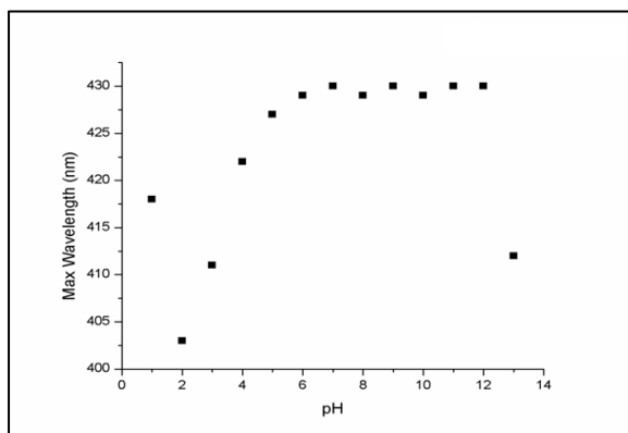
Fig 3: Changes in \lambda_{\max} value with Respect to pH Value
